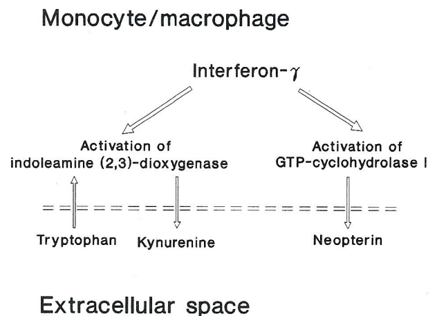
Fig. 1. Interferon- \gamma activates guanosine triphosphate-(GTP)-cyclohydrolase I in human monocytes/macrophages which leads to the formation of large amounts of neopterin. At the same time it induces indoleamine (2,3)-dioxygenase in a variety of cells which degrades tryptophan via the kynurenine pathway, with kynurenine being one of its first products.
