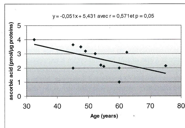
Figure 6. ^{14}\text{C} Ascorbic acid intracellular transport in Human Normal Fibroblasts (lifting), n=12 (M. Dumas courtesy).
